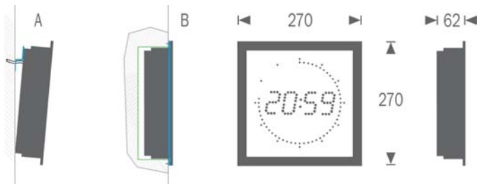
Wallmount case (A) with bracket provided or flush mount (B) with bracket provided.
